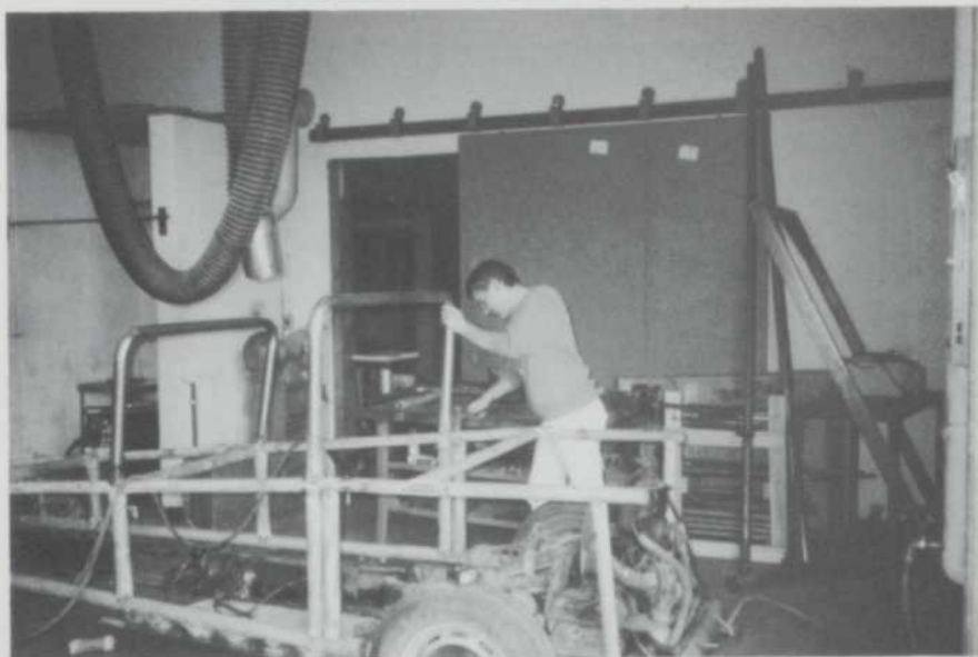
Ryan Prechtel works on his and Chad Hardin's Weld Tech. project, the Dune Buggy.
